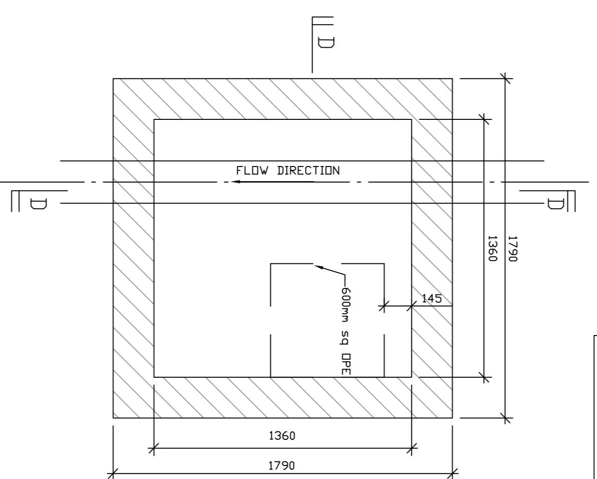
MANHOLE DETAIL FOR PIPE DIAMETERS DEPTH TO INVERT 1M TO 3M
