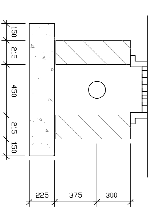
TYPICAL GULLY SECTION SCALE 1:20
