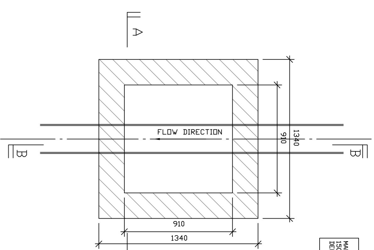
MANHOLE DETAIL FOR PIPE DIAMETERS DEPTH TO INVERT LESS THAN 1M
